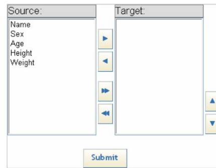
Figure 4: Altered DualListSelector
