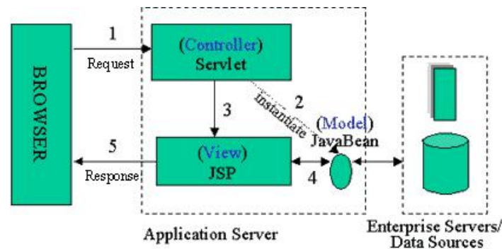
Figure 2: JSP Model 2 architecture
