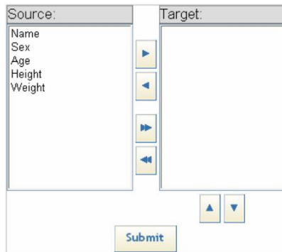
Figure 3: Default DualListSelector
